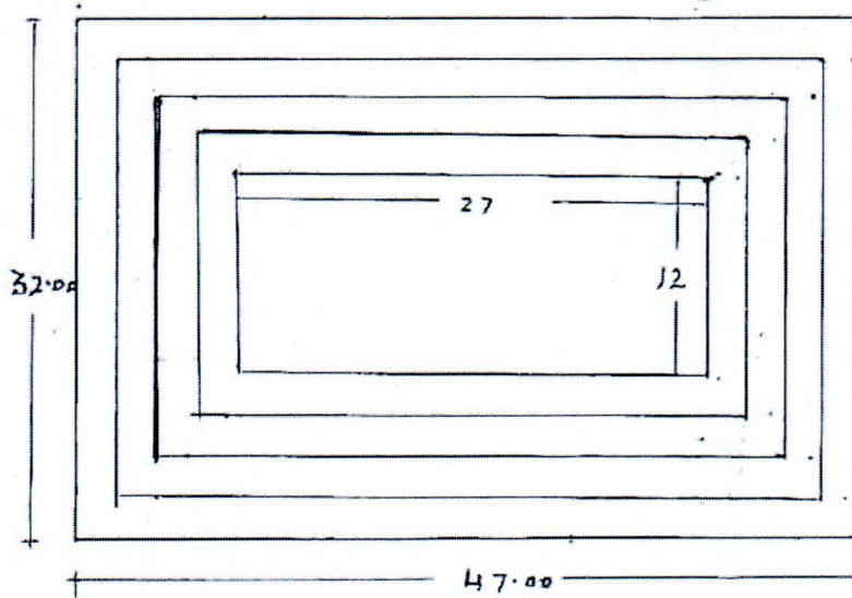
Excavation Plan of Pond Matiadand
