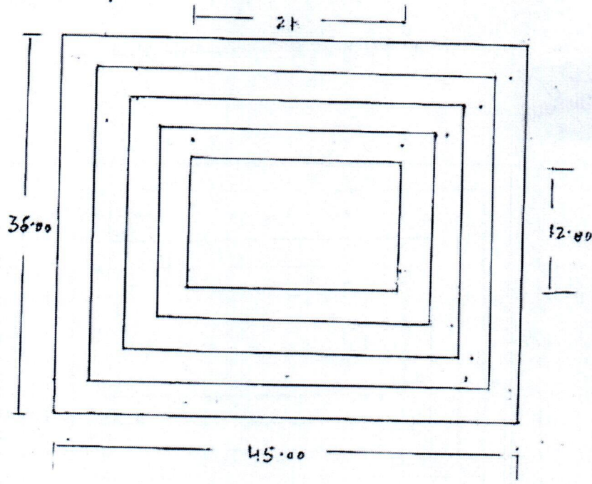
Excavation Plan OF Pond Thiatola/Runga
